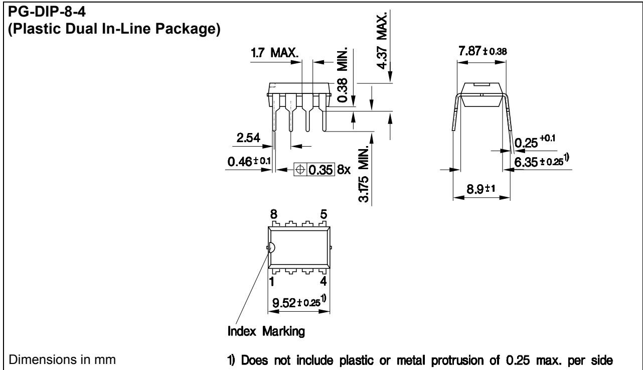
Figure 17 PG-DIP-8-4 Outline Dimension
