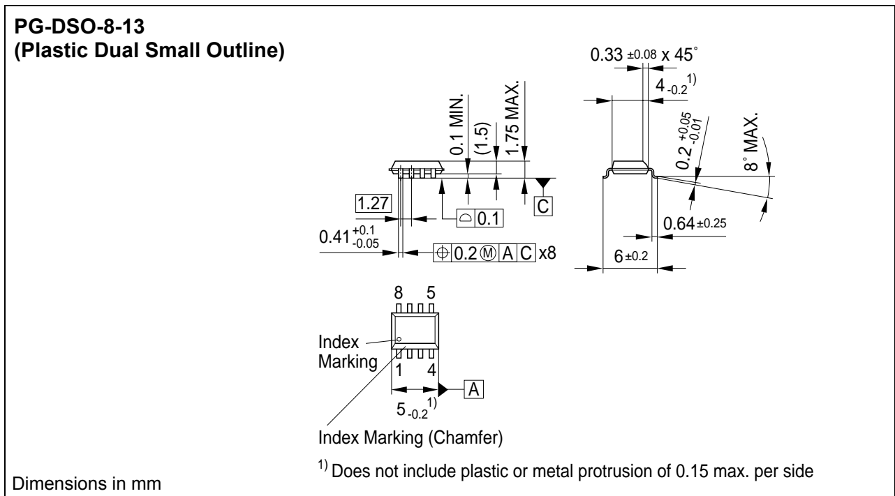
Figure 18 PG-DSO-8-13 Outline Dimension
