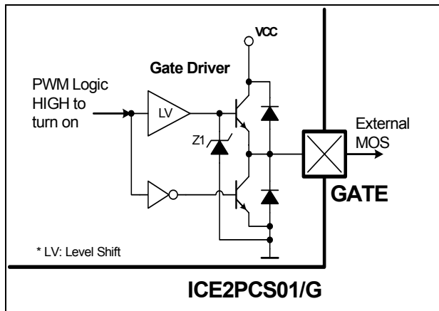
Figure 16 Gate Driver
